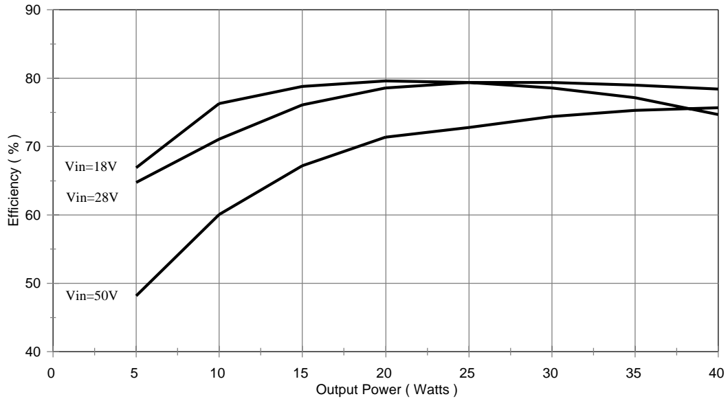
M3G280512T Efficiency vs Line and Load
