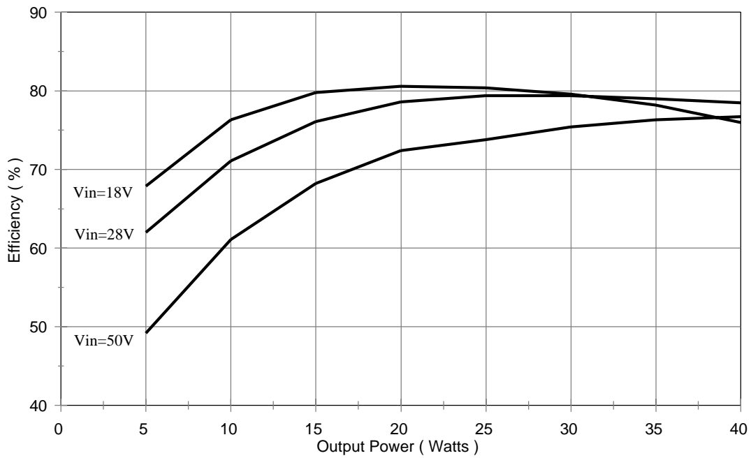
M3G280515T Efficiency vs Line and Load
